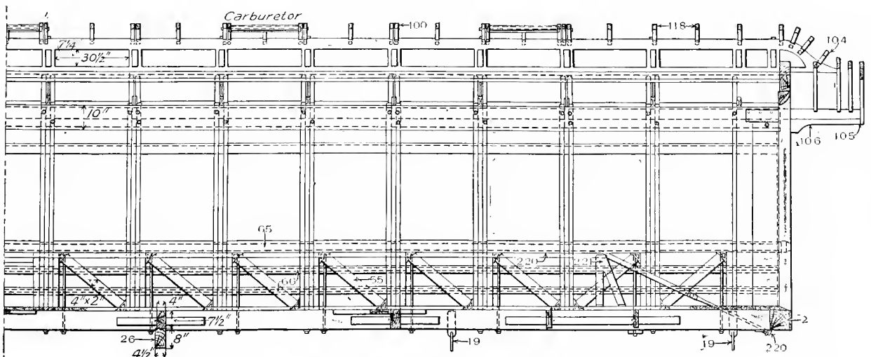
Fig. 440. Side Elevation showing Framing.
